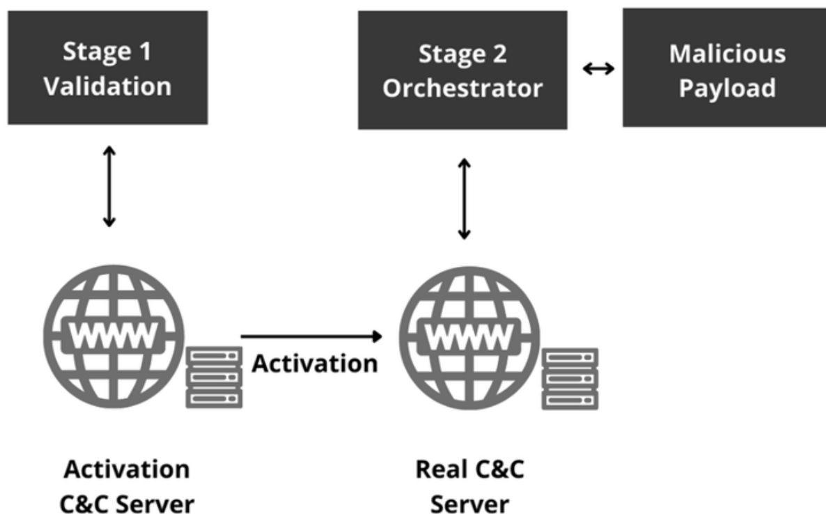
Fig: The architecture of ShadowPad backdoor
